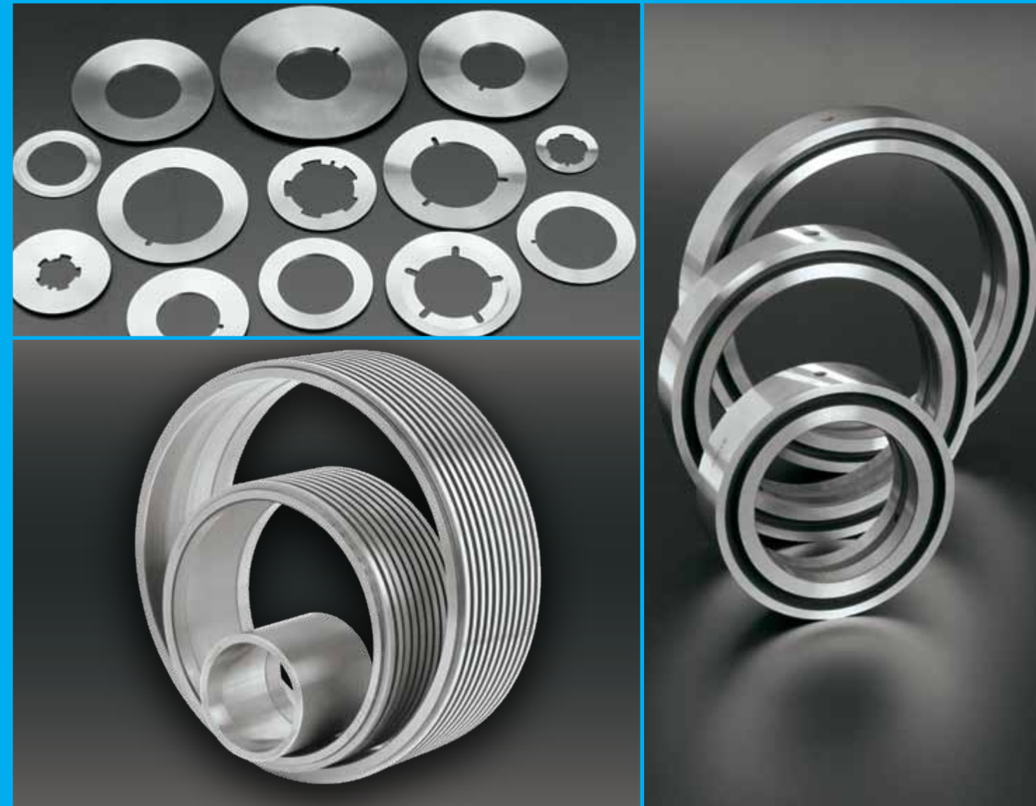
Top slitter Knives | Bottom slitter Knives | Multi Knife blocks
